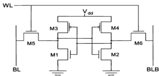
Conventional 6T SRAM cell
