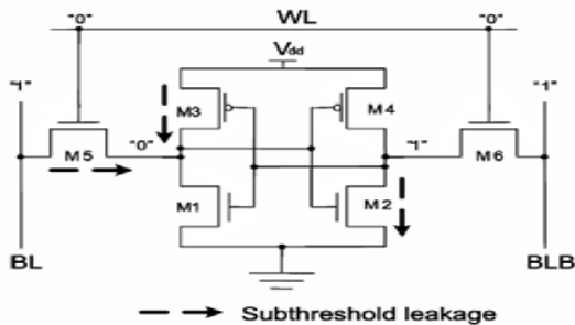
Sub-Threshold leakage current in SRAM cell
