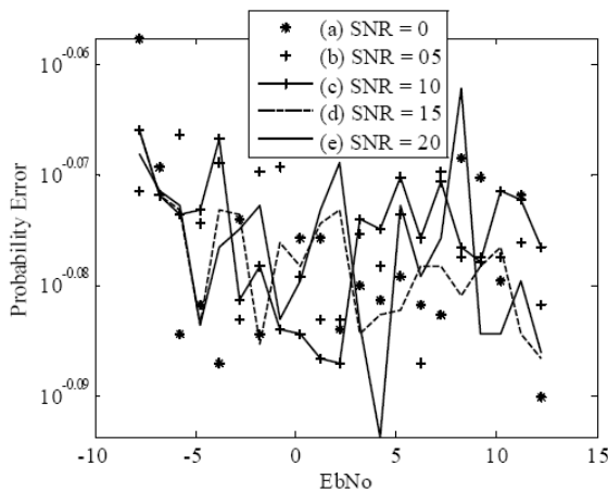
Figure 4: Performance Analysis of QAM Modulation in Rayleigh fading Channel for SDR at different SNR
