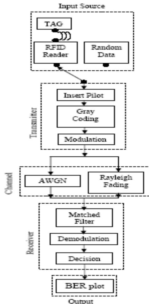
Figure 1: Block diagram for a system Model
