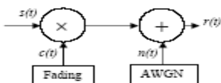
Figure 2: Transmission channel model
