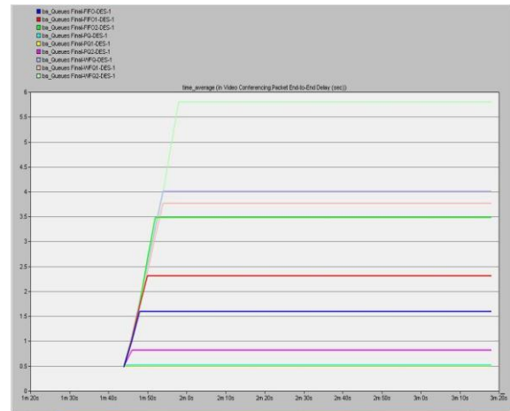
Figure 3.6 Video Conference Packet End to End Delay
