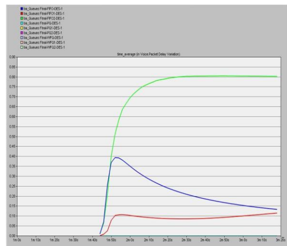
Figure 3.7 Voice Delay Variation
