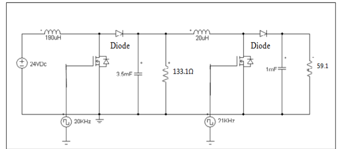
Fig. 2 Dual stage Boost Power Converter
