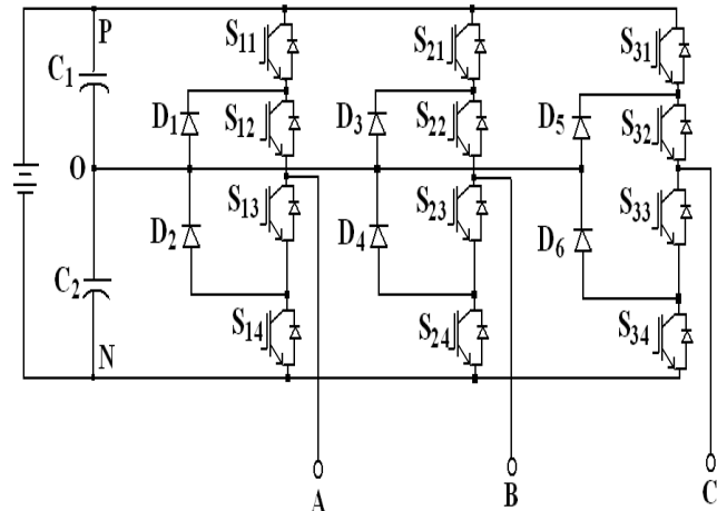
Fig no. 01 : Schematic diagram of three-level inverter
