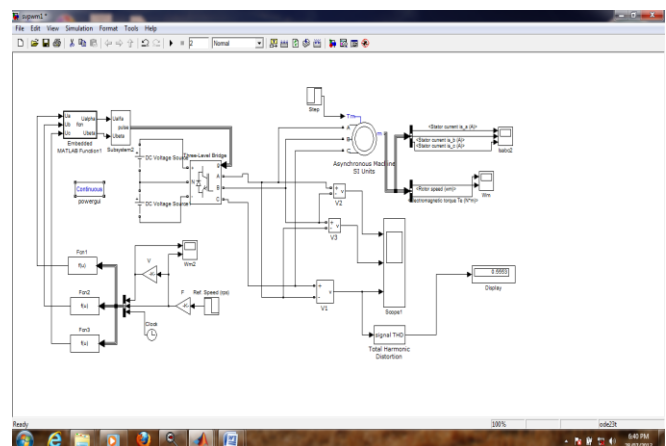
Fig.3.1 : SVPWM based speed control of induction motor v/f control
