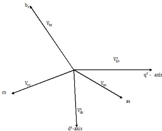
Fig. 2.1 Stationary Frame a-b-c to d s -q s Axes Transform motion
